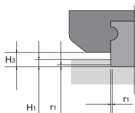
LM rail section
