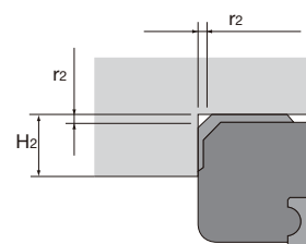
LM block section
