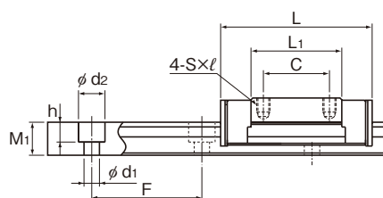
SRS9XM/9XN/12M/12N
