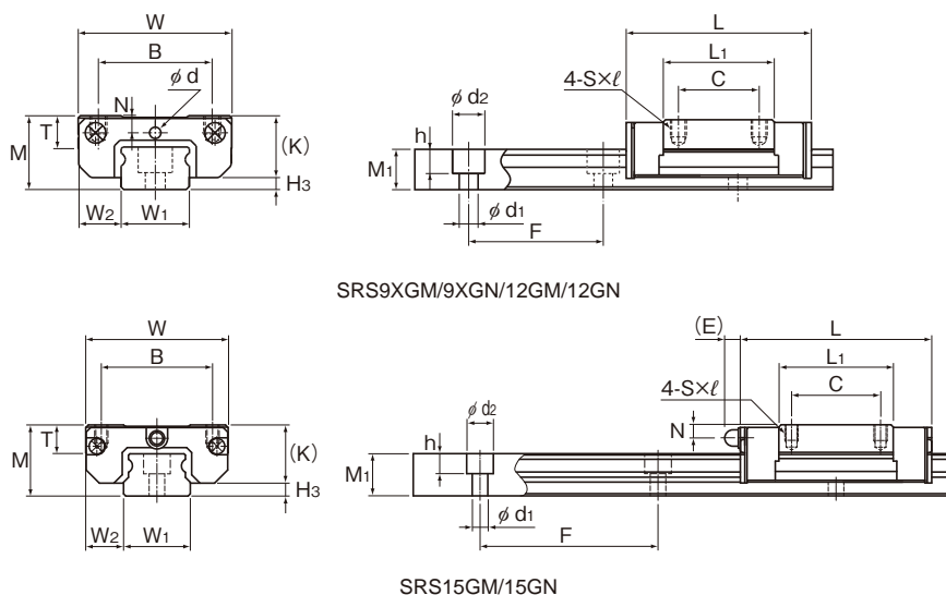
SRS15GM/15GN
