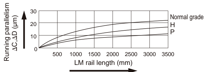
Fig.3 LM Rail Length and Running Parallelism (HSR/SR/SHS/SSR)
