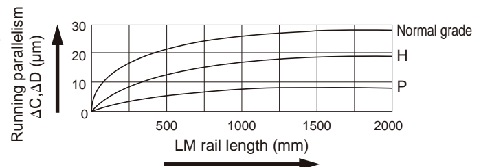
Fig.4 LM Rail Length and Running Parallelism (SRS-G/SRS)
