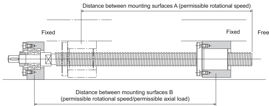
Fig. 1: Screw Shaft Mounting Method: Fixed - Free
