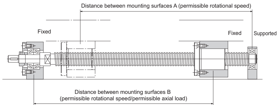
Fig. 2: Screw Shaft Mounting Method: Fixed - Supported
