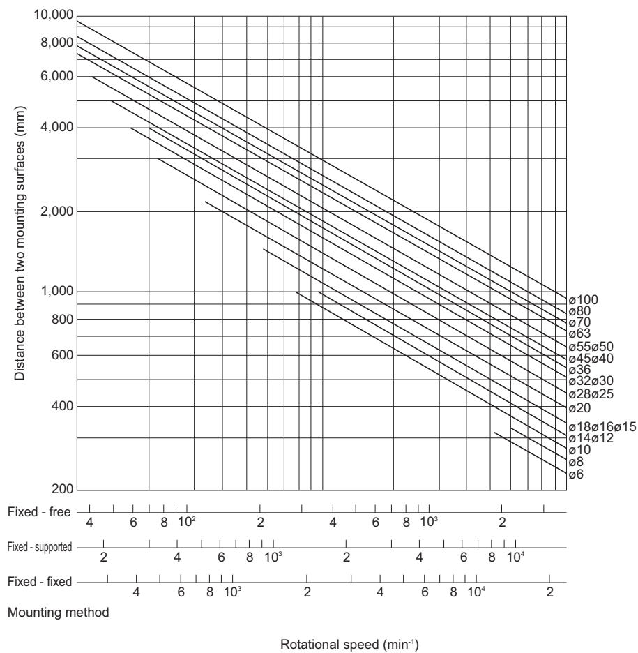
Fig. 6: Permissible Rotational Speed Diagram
