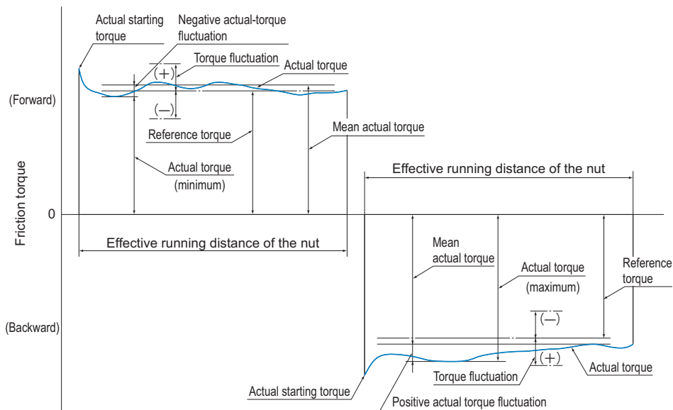
Fig. 7: Preload Torque Terminology
